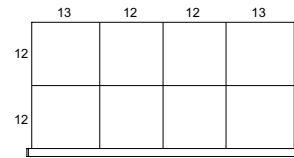
R_JG-A0304__ 8 COMPARTMENTS
