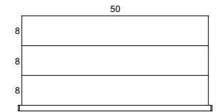
R_JG-B0200__ 3 COMPARTMENTS
