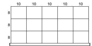
R_JG-A0410__ 15 COMPARTMENTS
