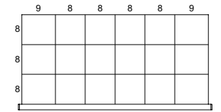
R_JG-A0512__ 18 COMPARTMENTS
