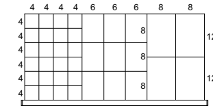
R_JG-D0828__ 37 COMPARTMENTS
